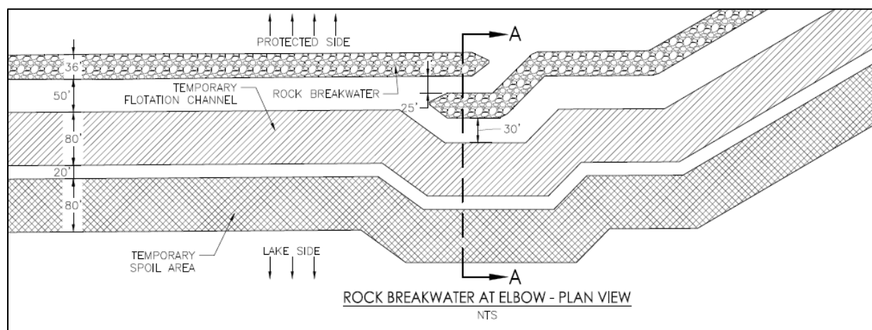
Figure 9: Proposed Rock Elbows
